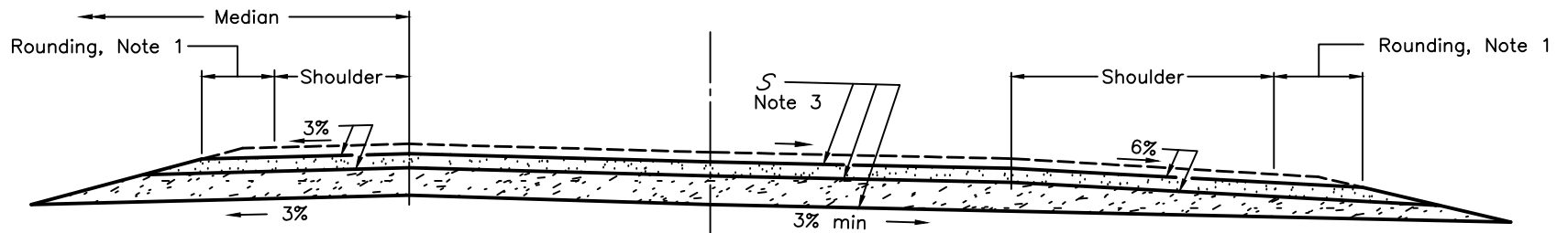
SUPERELEVATED SECTION MEDIAN ON HIGH SIDE
