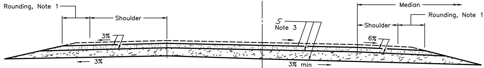
SUPERELEVATED SECTION MEDIAN ON LOW SIDE
