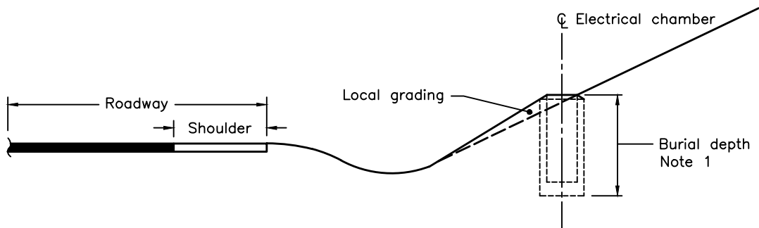
ELECTRICAL CHAMBER IN CUT
