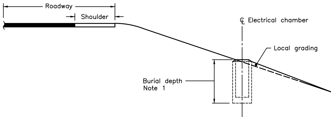
ELECTRICAL CHAMBER IN FILL
