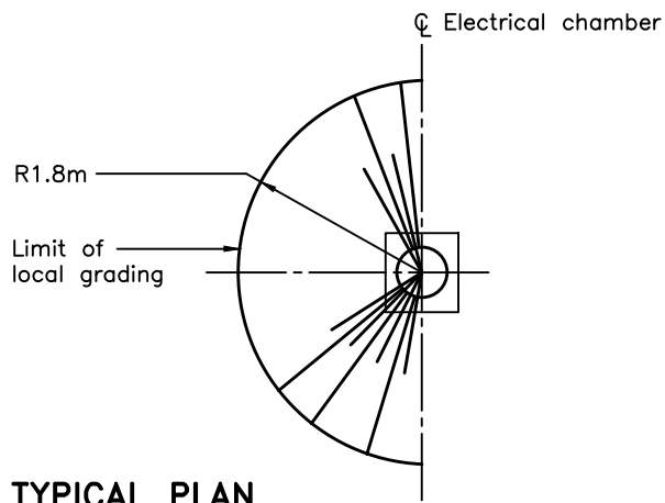
TYPICAL PLAN
