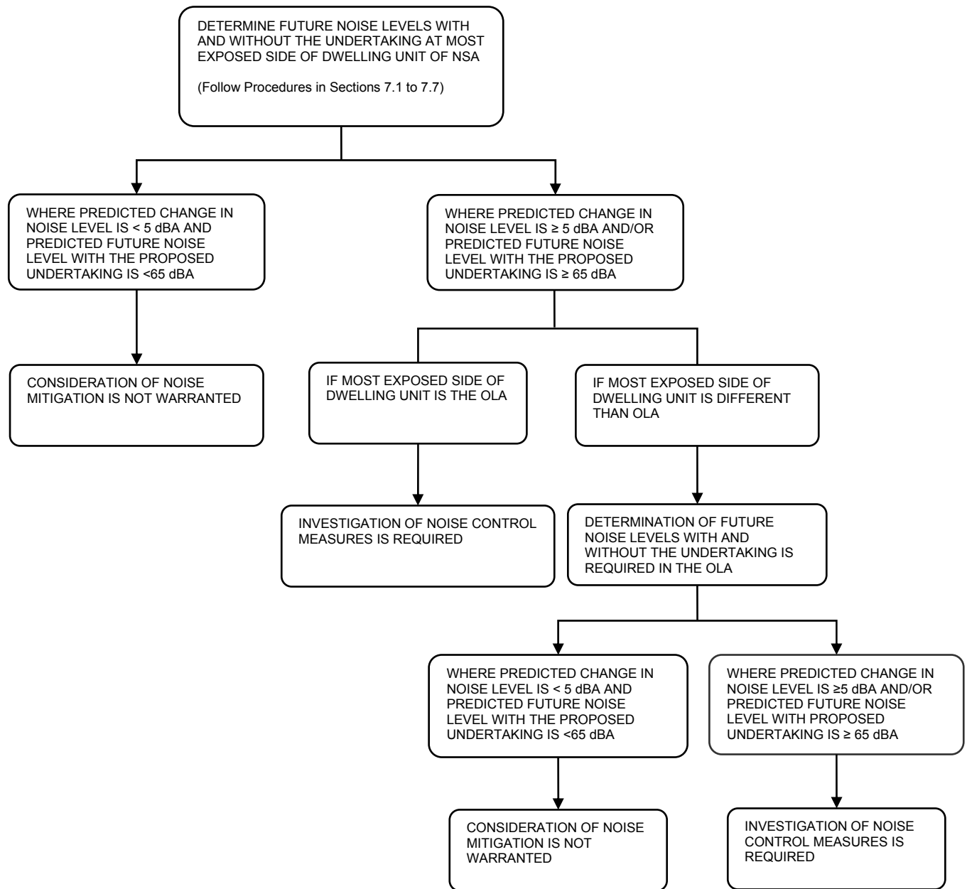
Figure 7.1 Preliminary Assessment of Mitigation
