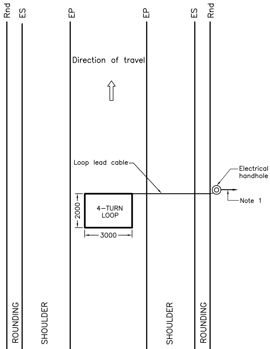
PLAN VIEW
