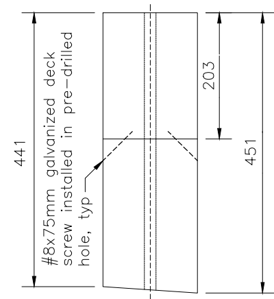
WOODEN OFFSET BLOCK 4
