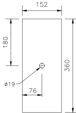
WOODEN OFFSET BLOCKS 1 THROUGH 4 ELEVATION
