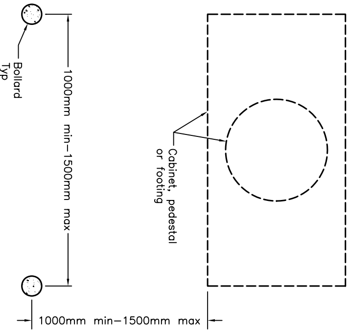
BOLLARDS AND FIELD EQUIPMENT SITE LAYOUT Note 1 PLAN
