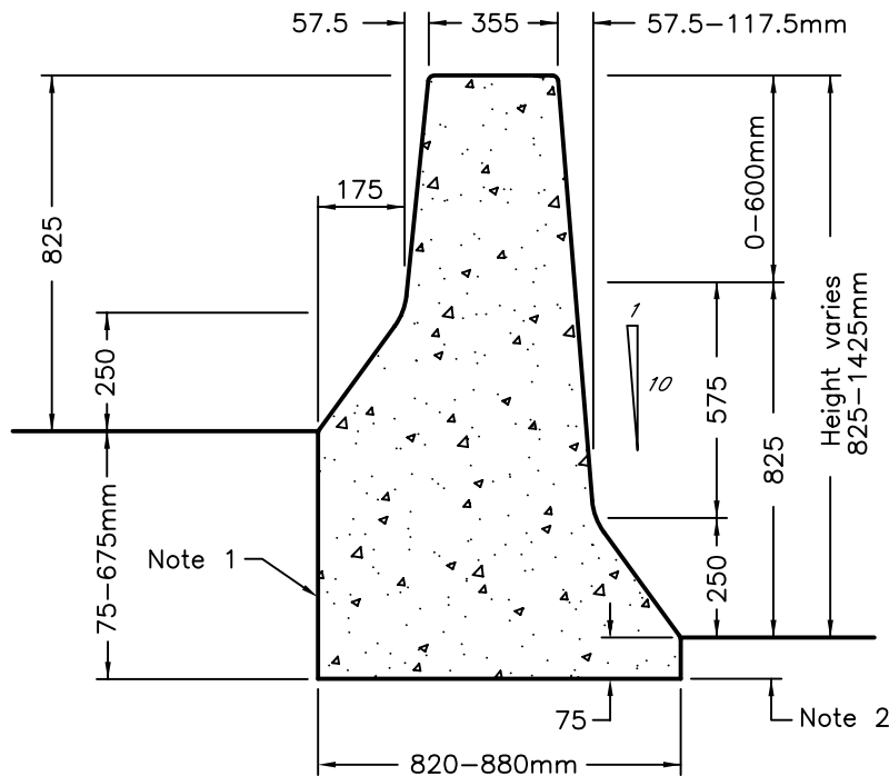
TYPE C-1 ASYMMETRIC SECTION
