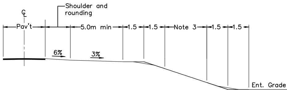
TYPICAL PROFILE IN FILL
