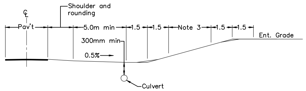
TYPICAL PROFILE IN CUT
