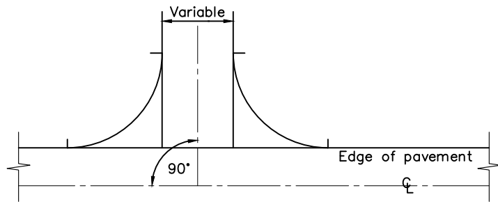
TYPICAL ENTRANCE
